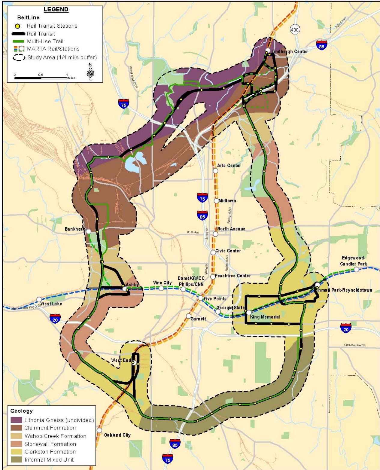
Figure 2.16-1: Geologic Formations
